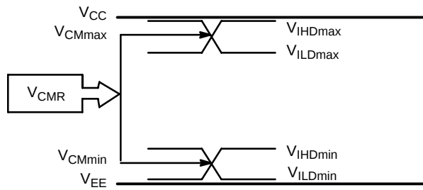
Figure 11. V_{CM} Diagram
