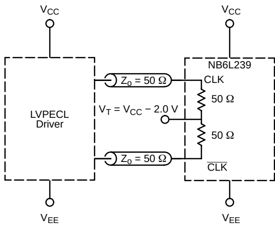
Figure 12. LVPECL Interface
