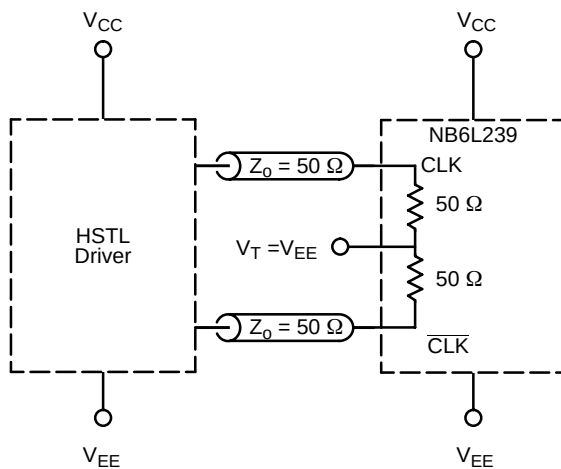
Figure 15. Standard 50 \Omega Load HSTL Interface
