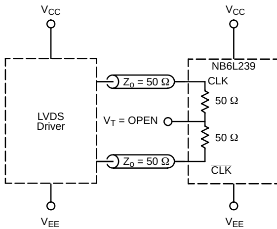
Figure 13. LVDS Interface
