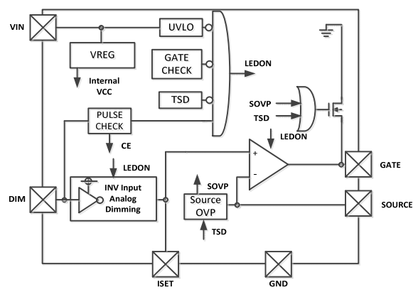
R1580N003A Block Diagram
