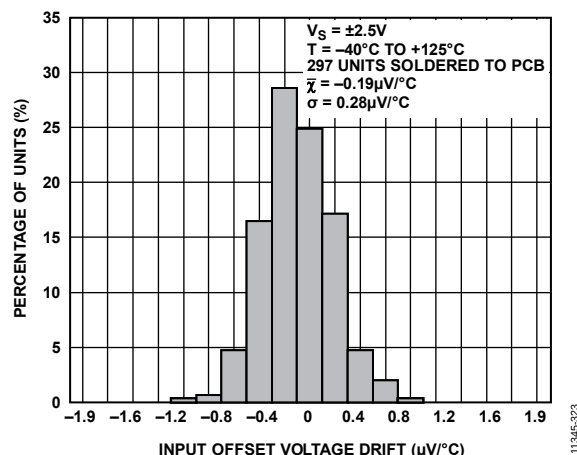
Figure 29. Input Offset Voltage Drift Distribution
