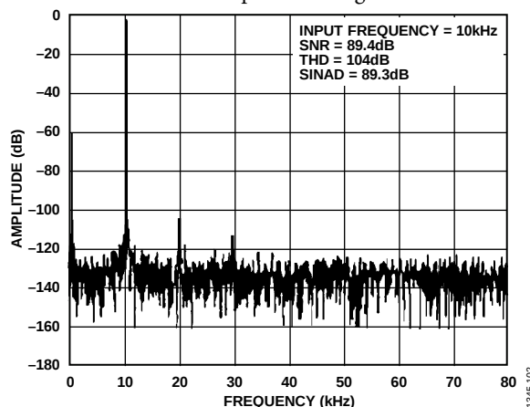
Figure 2. FFT Plot for the Circuit Configuration in Figure 1
