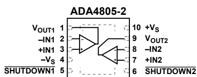
Figure 6. 10-Lead LFCSP Pin Configuration
