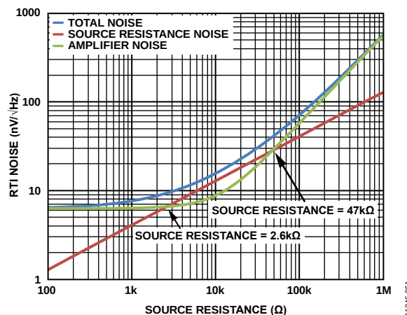
Figure 55. RTI Noise vs. Source Resistance
