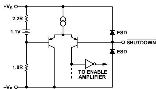
Figure 53. Shutdown Circuit
