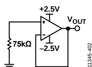
Figure 47. Current Noise Test Circuit (See Figure 23)
