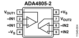
Figure 7. 8-Lead MSOP Pin Configuration
