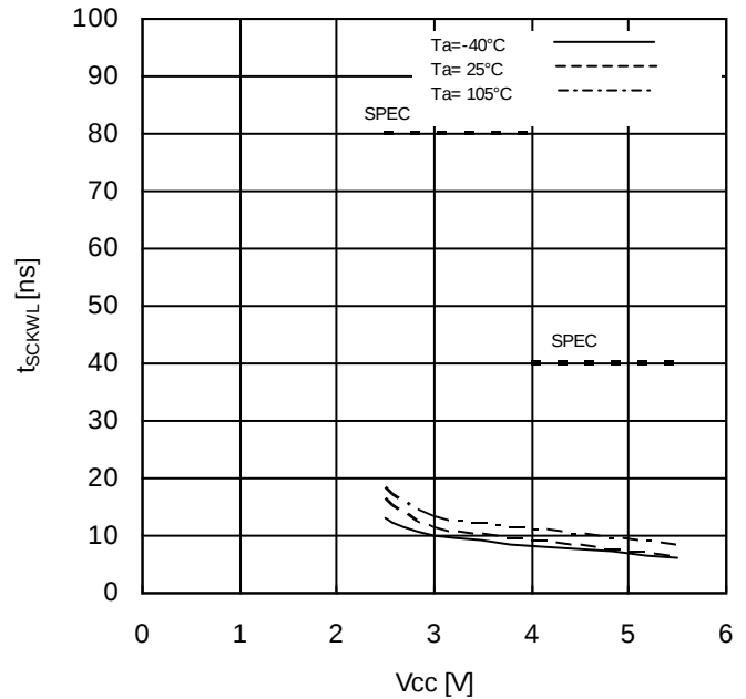
Figure 16. SCK Low Time vs Supply Voltage
