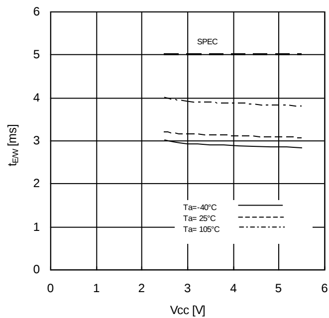
Figure 30. Write Cycle Time vs Supply Voltage
