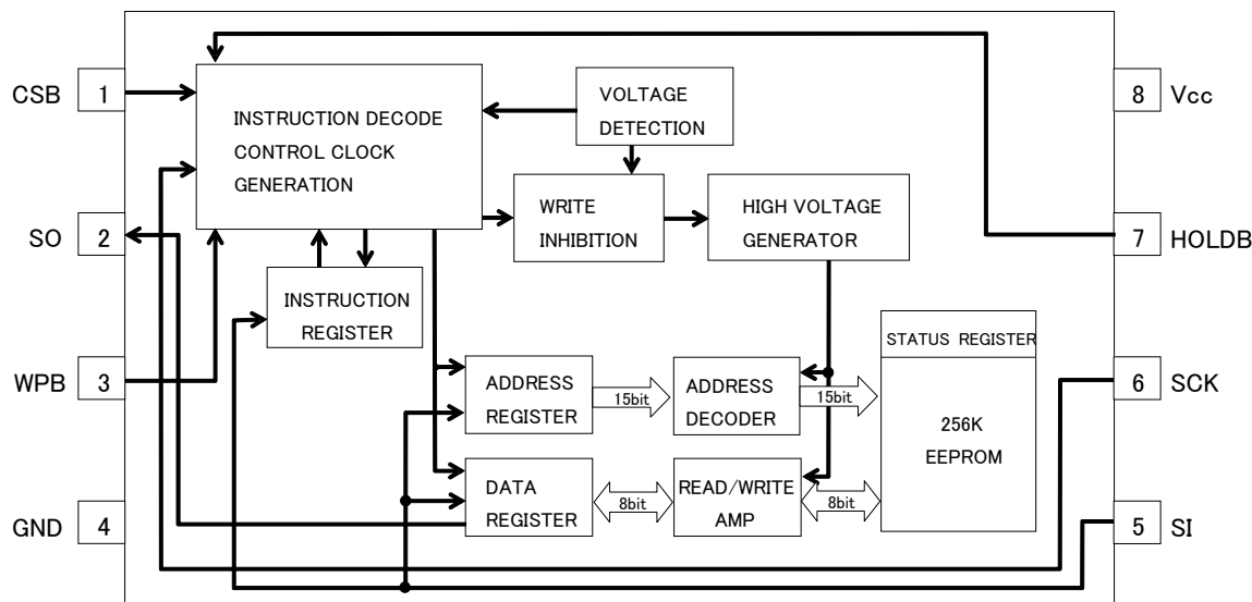
Figure 3. Block Diagram
