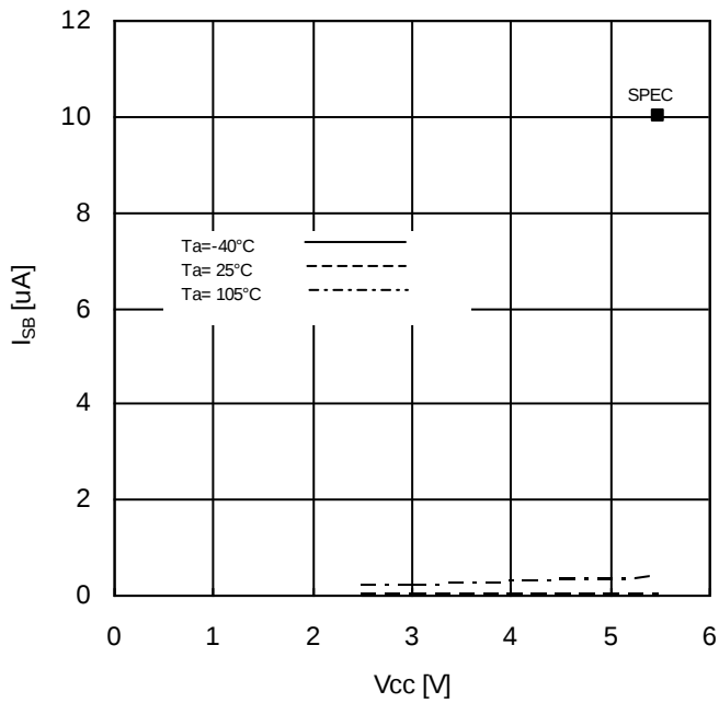
Figure 13. Standby Current vs Supply Voltage
