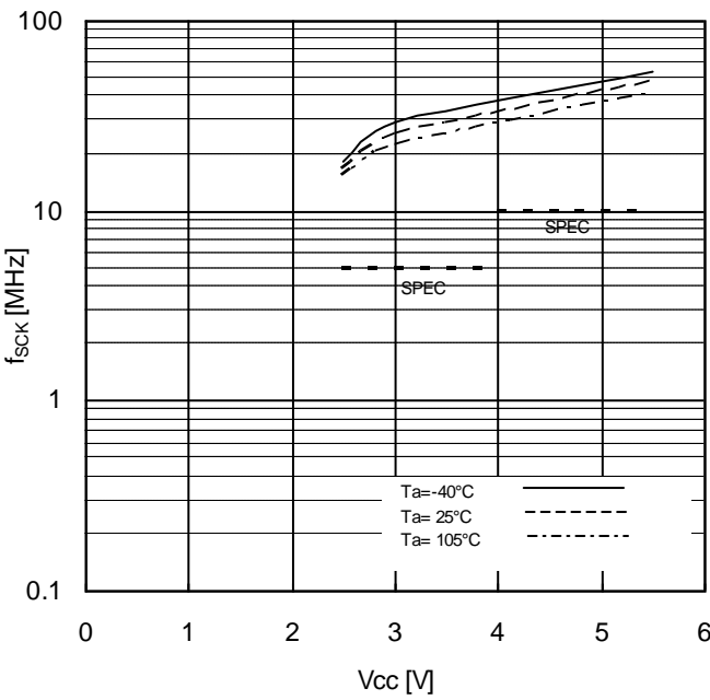
Figure 14. SCK frequency vs Supply Voltage
