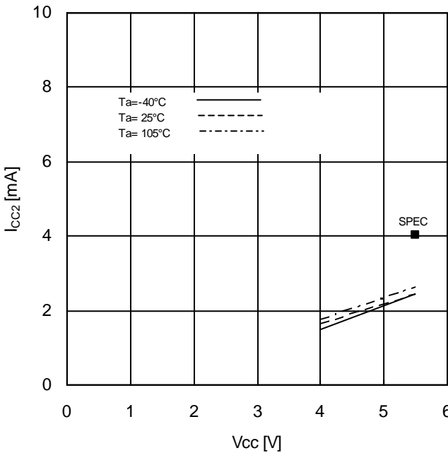
Figure 12 Supply Current (Read)vs Supply Voltage (f sck =10MHz)
