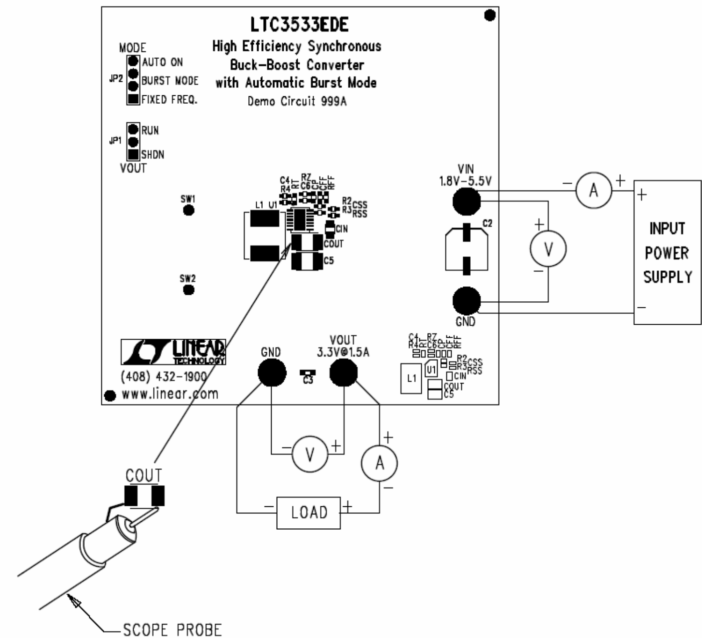
Figure 1. Proper Measurement Equipment Setup
