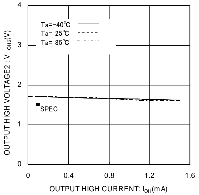
Figure 9. Output high voltage2 V_{OH2} ( V_{CC}=1.7\text{V} )
