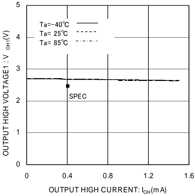
Figure 8. Output high voltage1 V_{OH1} ( V_{CC}=2.7\text{V} )
