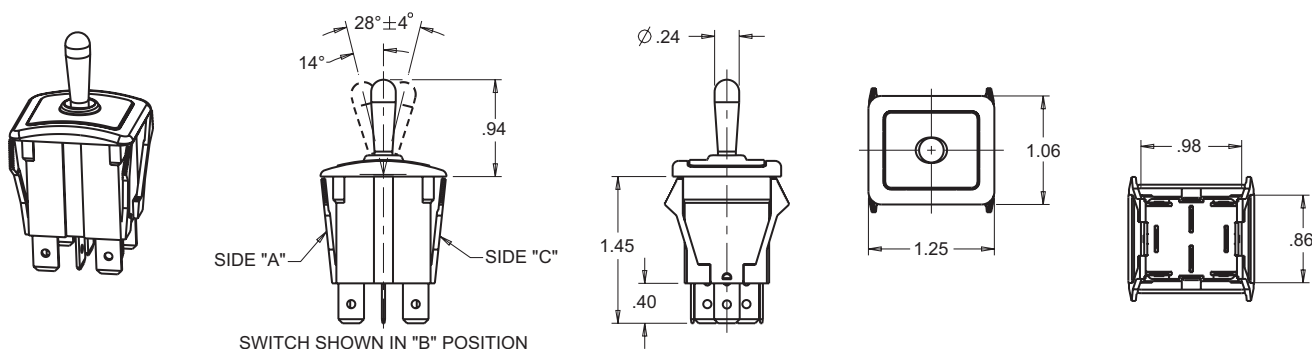
SWITCH SHOWN IN "B" POSITION
