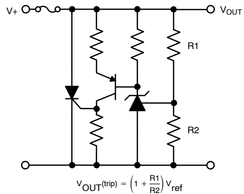
Figure 29. SRC Crowbar
