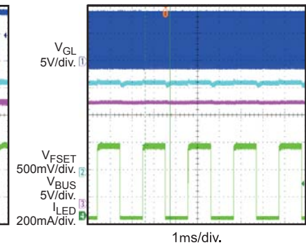
PWM Dimming, 50%, 480Hz
