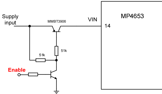
Figure 4—MP4653 Enable control circuit
