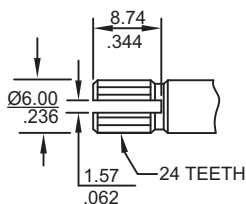
K - Slot & Knurled
