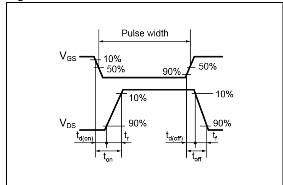
Fig. 2-2 SWITCHING WAVEFORMS
