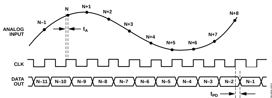
Figure 2. Timing Diagram
