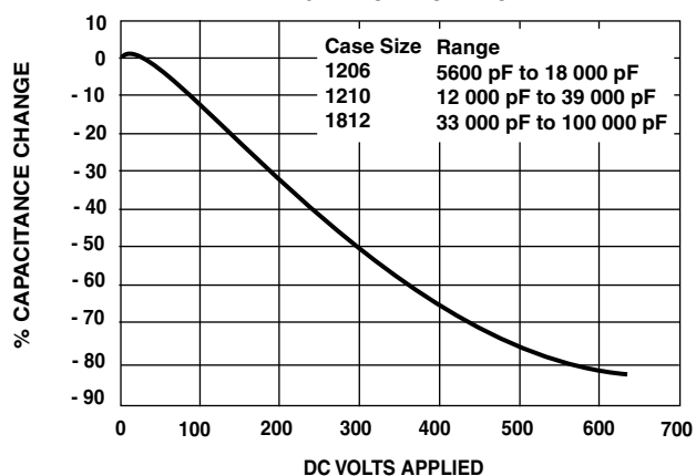
VOLTAGE COEFFICIENT OF CAPACITANCE HIGHER CAPACITANCE
