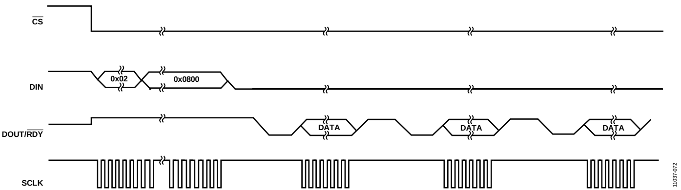
Figure 48. Continuous Read Mode
