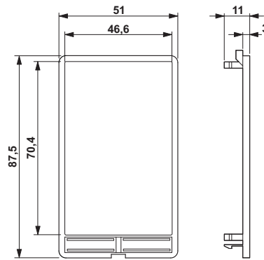
Dummy plate
