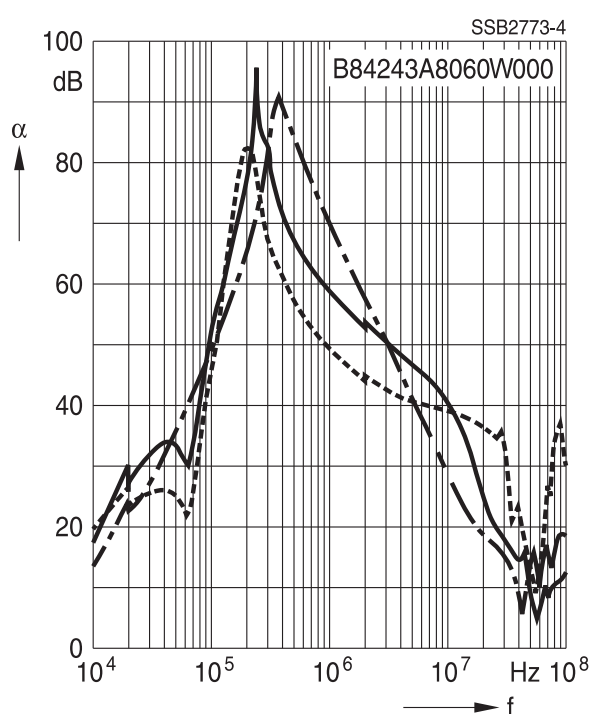
Filter for 60 A
