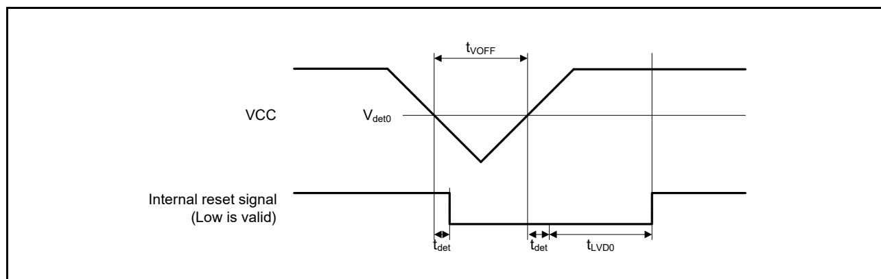
Figure 5.84 Voltage Detection Circuit Timing ( V_{\text{det0}} )
