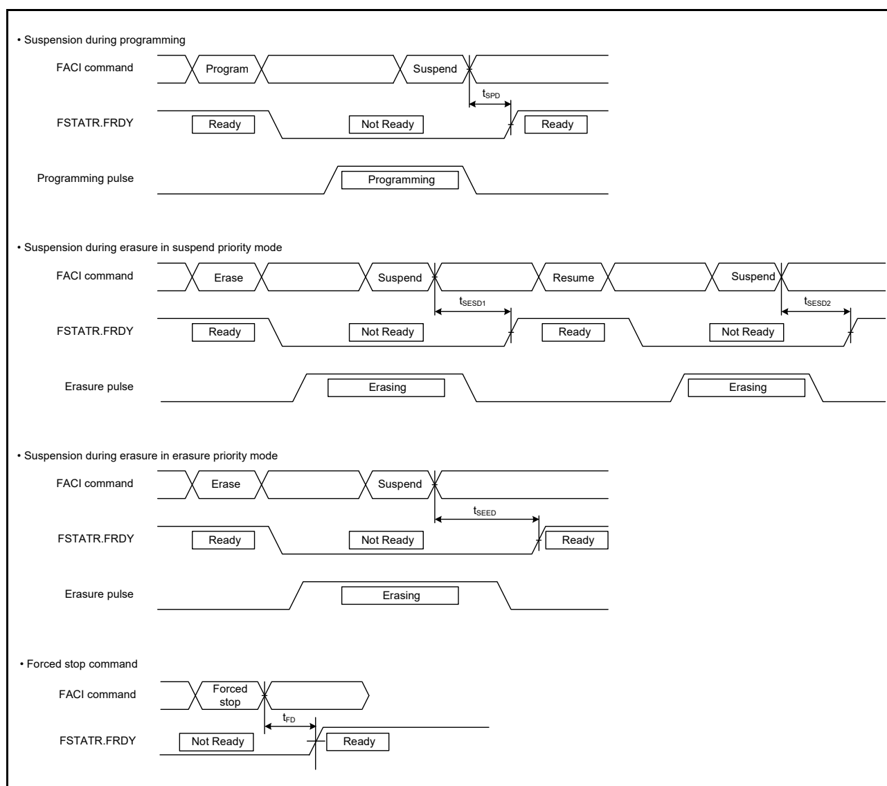
Figure 5.89 Flash Memory Programming/Erase Suspension Timing
