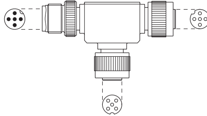
Layout of connector pin assignments
