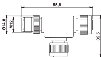
M12 T-distributor
