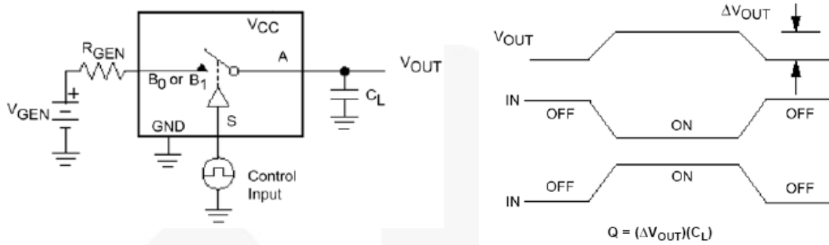
Figure 6. Charge Injection
