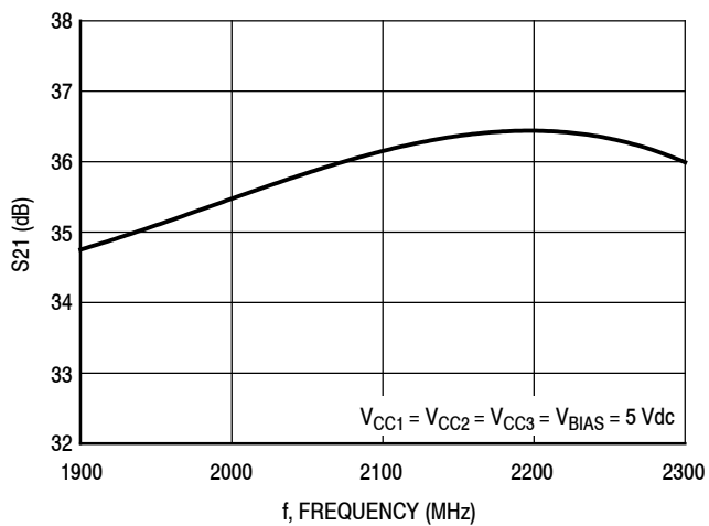
Figure 15. S21 versus Frequency
