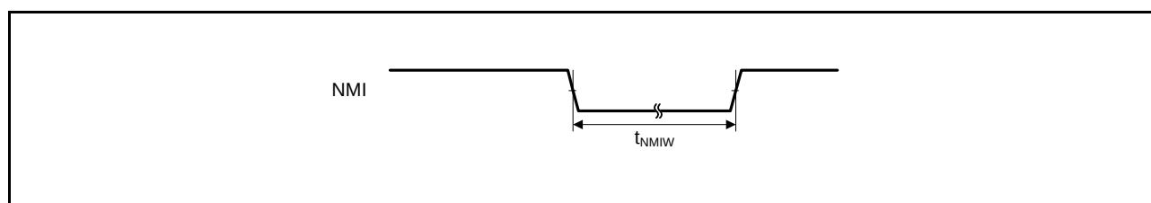
Figure 5.32 NMI Interrupt Input Timing
