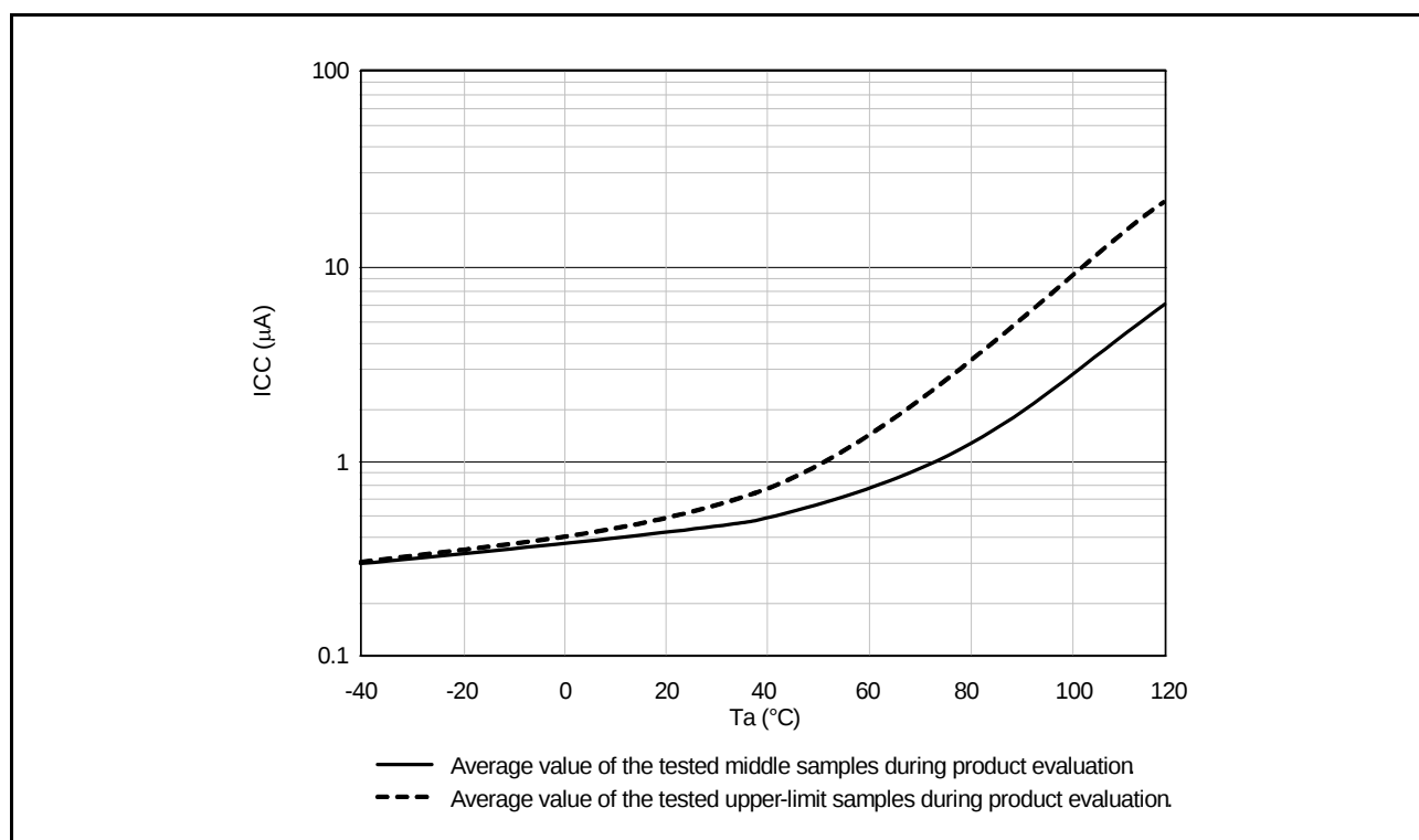
Figure 5.2 Temperature Dependency in Software Standby Mode (Reference Data)
