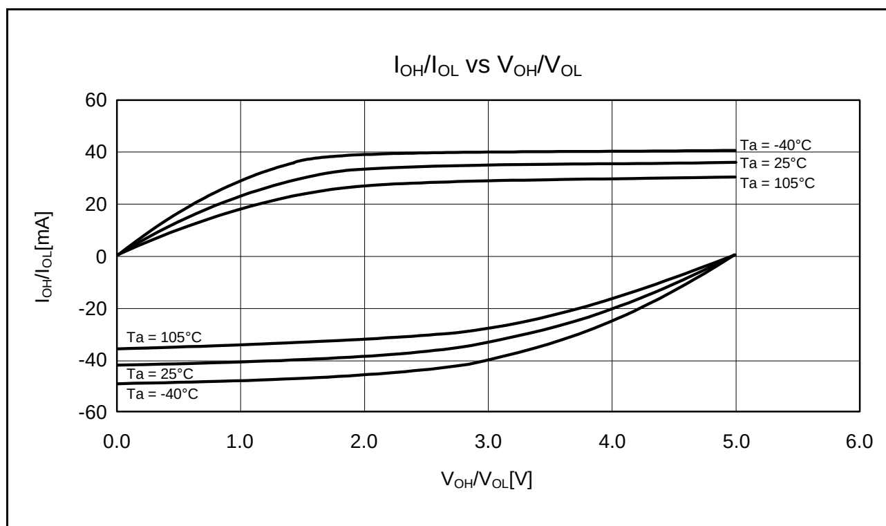
Figure 5.6 V_{OH}/V_{OL} and I_{OH}/I_{OL} Temperature Characteristics at V_{CC} = 5.0 V when Normal Output is Selected (Reference Data)
