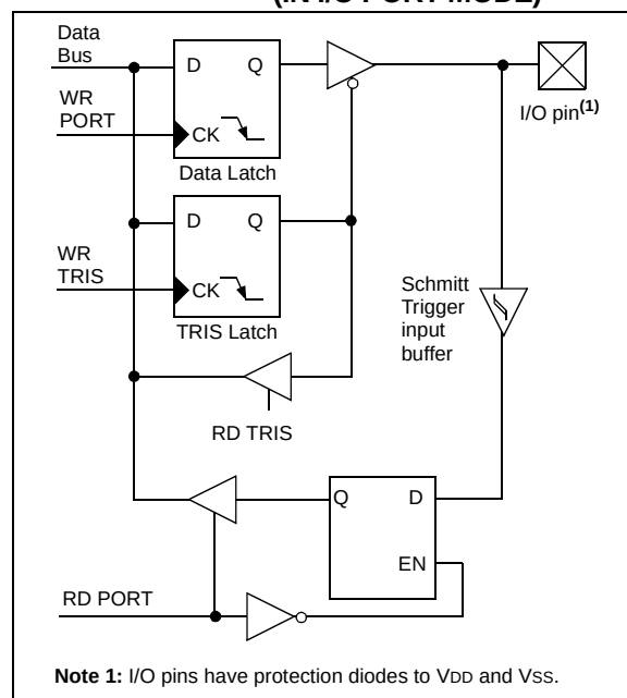
FIGURE 4-7: PORTE BLOCK DIAGRAM (IN I/O PORT MODE)
