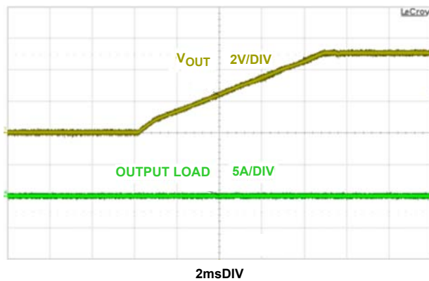
FIGURE 15. START-UP AT 0A LOAD CONDITION
