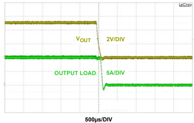
FIGURE 18. SHUTDOWN AT 10A LOAD CONDITION
