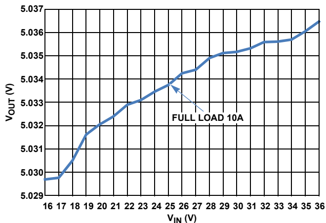
FIGURE 11. LINE REGULATION AT FULL LOAD DEM MODE
