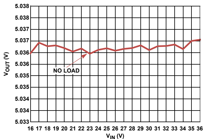
FIGURE 8. LINE REGULATION AT NO LOAD CCM MODE
