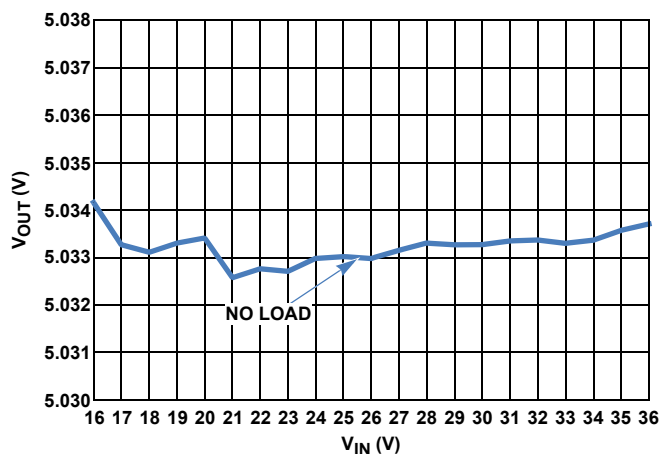
FIGURE 9. LINE REGULATION AT NO LOAD DEM MODE
