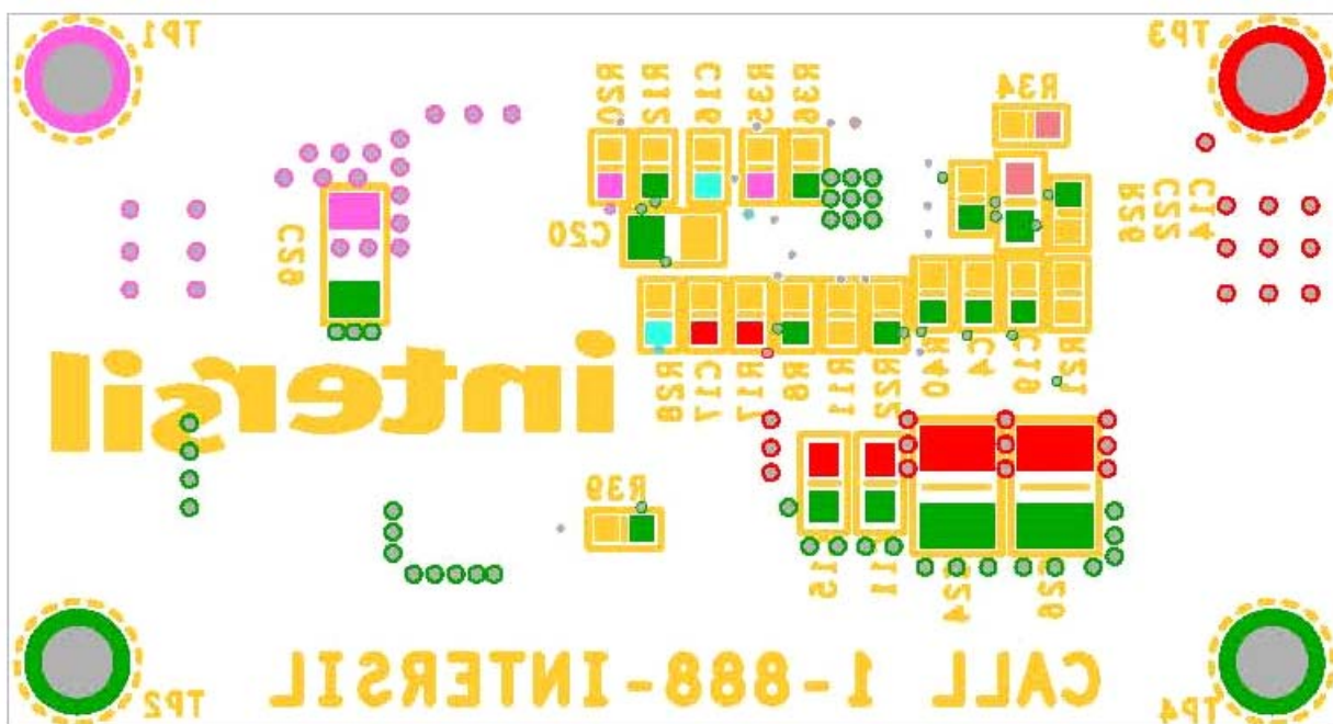
FIGURE 23. BOTTOM
