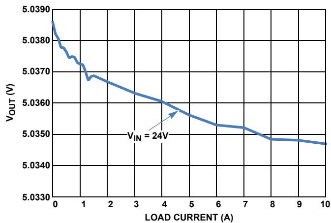
FIGURE 7. V_{OUT} LOAD REGULATION AT DEM MODE
