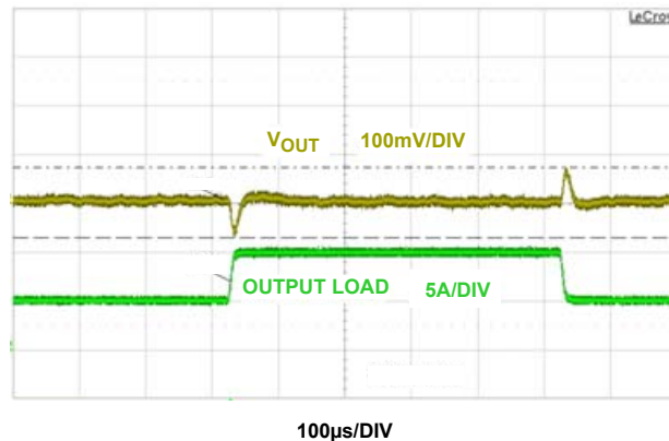
FIGURE 14. LOAD TRANSIENT 5A TO 10A; 2A/µs AT CCM
