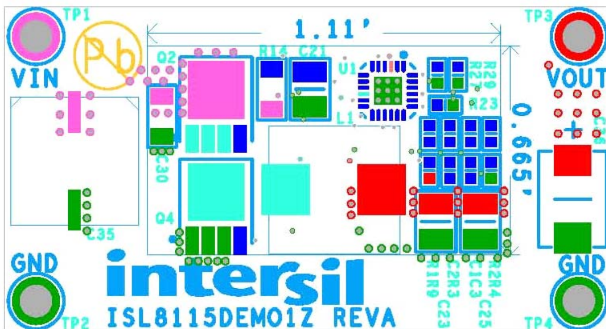
FIGURE 22. TOP
