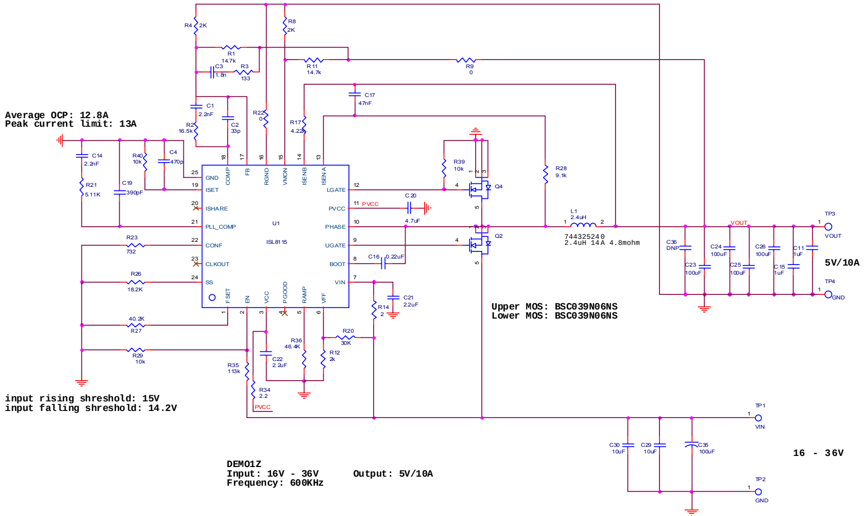
FIGURE 21. ISL8115DEMO1Z SCHEMATIC
