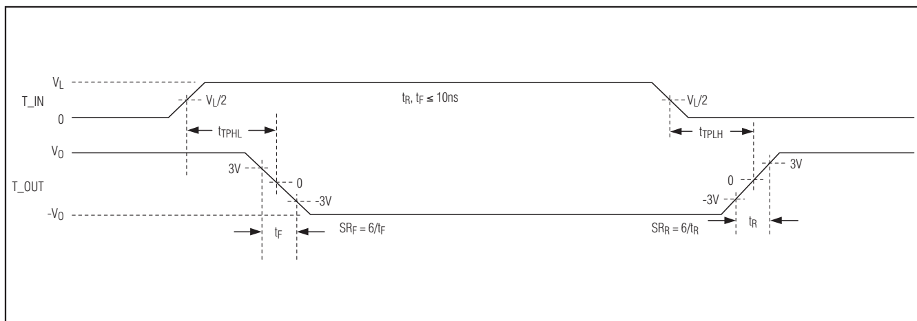
Figure 5. Transmitter Propagation Delay
