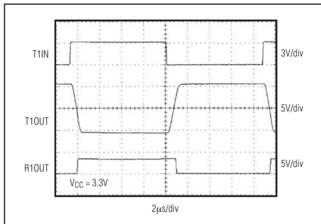
Figure 12. Loopback Test Results at 120kbps
