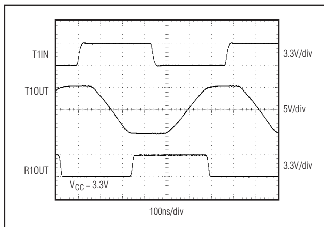
Figure 13. Loopback Test Results at 3Mbps
