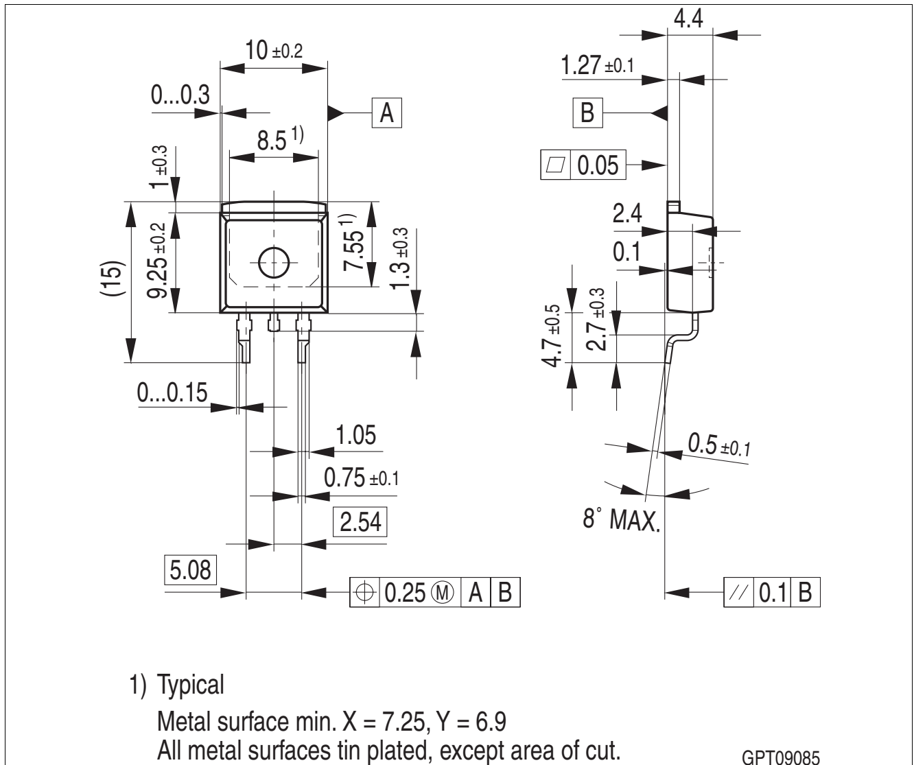
Figure 1 PG-TO263-3-2
