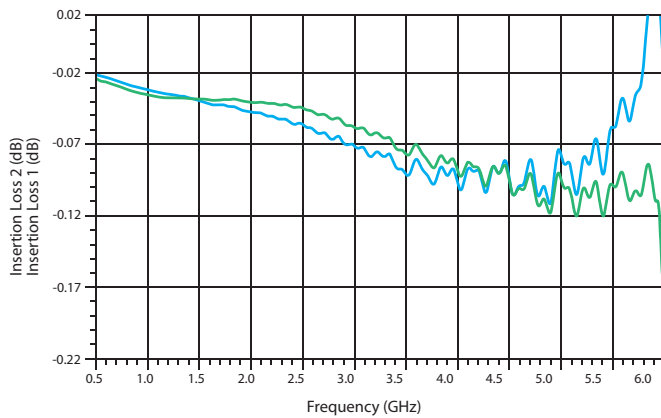
RF/RF Crossover – Insertion Loss
