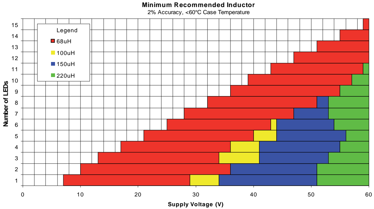
Figure 3 ZXLD1366QET5 Minimum Recommended Inductor (TSOT25)
