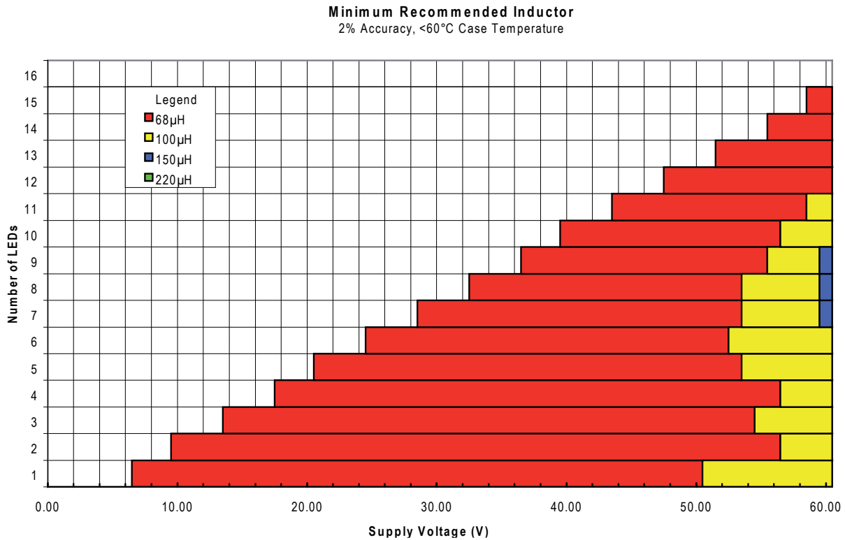
Figure 5 ZXLD1366 Minimum Recommended Inductor (U-DFN3030-6)
