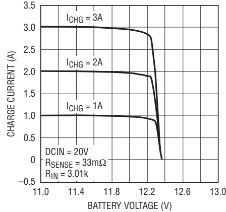
Charge Current Load Regulation
