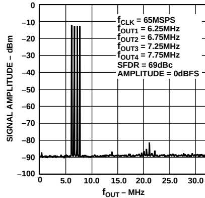
Figure 16. Four-Tone SFDR
