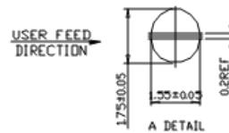
A DETAIL
