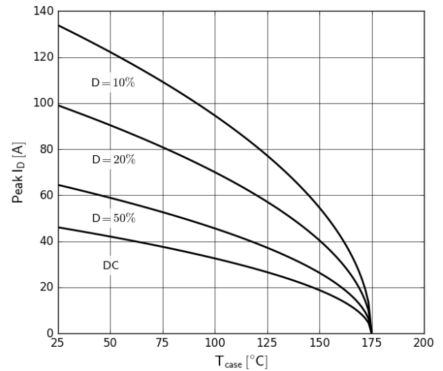
Figure 10. Current Derating
