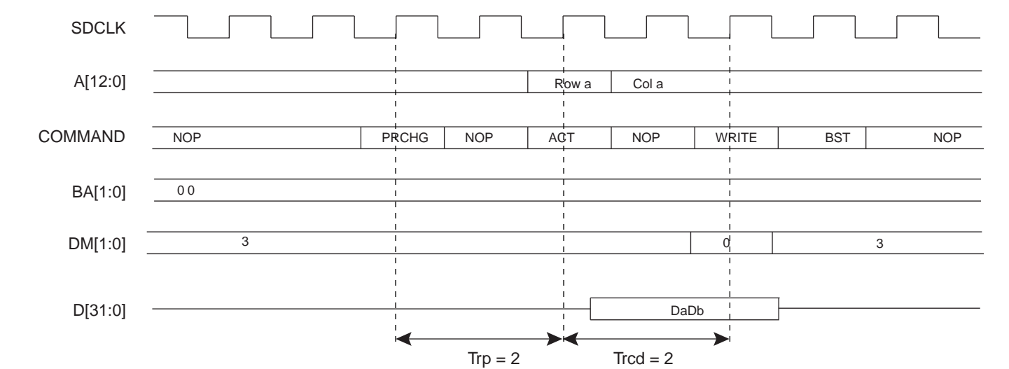
Figure 22-4. Single Write Access, Row Closed, SDR-SDRAM Device
