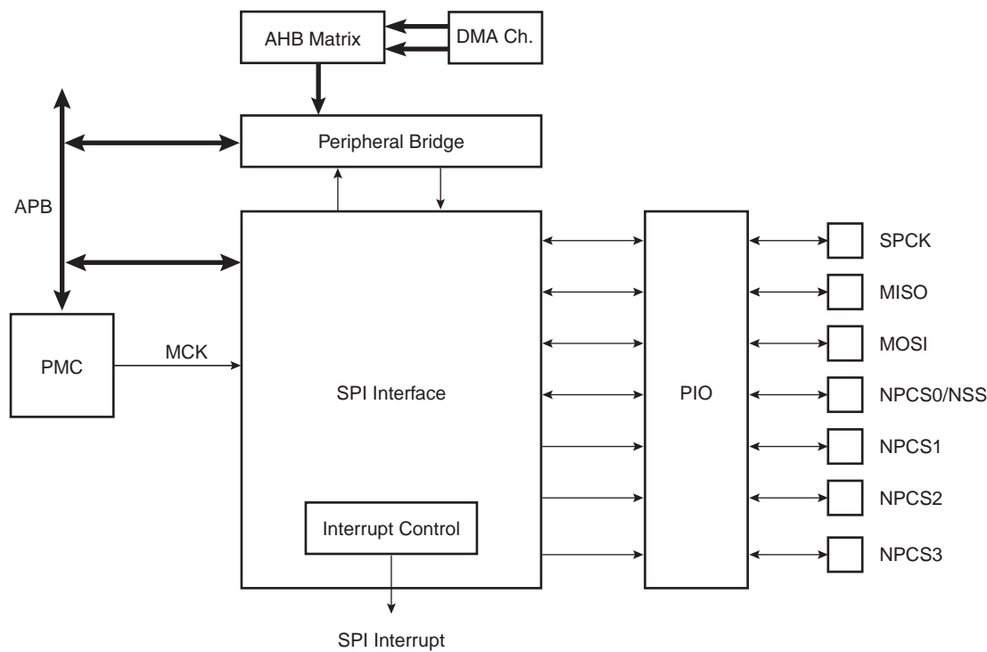
Figure 29-1. Block Diagram
