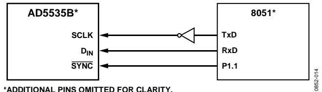
Figure 19. AD5535B-to-8051 Interface
