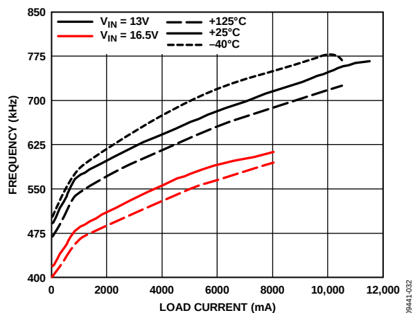
Figure 32. Frequency vs. Load Current, V_{OUT} = 1.0 \text{ MHz} , V_{OUT} = 0.8 V
