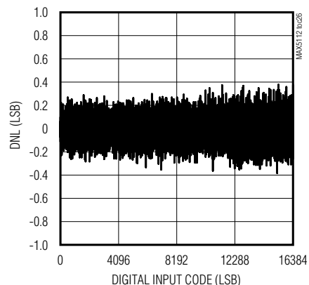
OP1 DIFFERENTIAL NONLINEARITY vs. DIGITAL INPUT CODE
