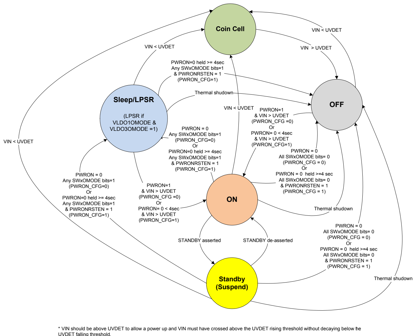
Figure 15. State diagram
