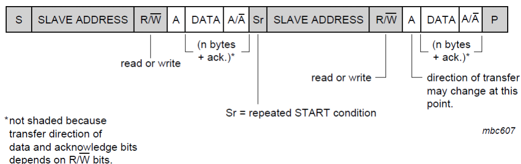
Figure 35. Read operation
