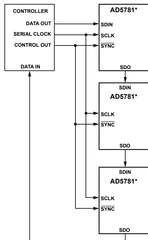
*ADDITIONAL PINS OMITTED FOR CLARITY. Figure 51. Daisy-Chain Block Diagram
