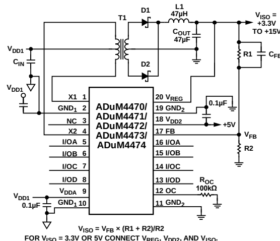
Figure 48. Single Power Supply
