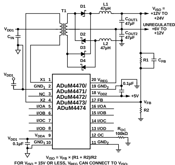
Figure 49. Doubling Power Supply
