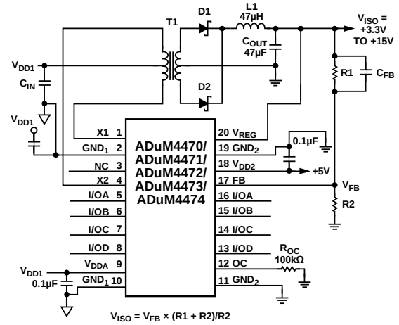
Figure 48. Single Power Supply
