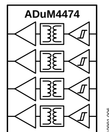
Figure 6. ADuM4474
