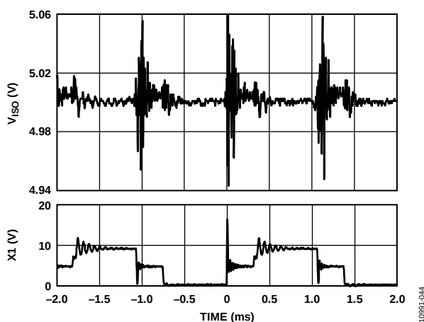
Figure 44. Typical V_{ISO} Output Ripple, 5 V Input to 5 V Output at 400 mA Load at 500 kHz f_{SW}
