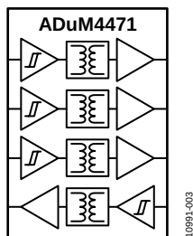
Figure 3. ADuM4471
