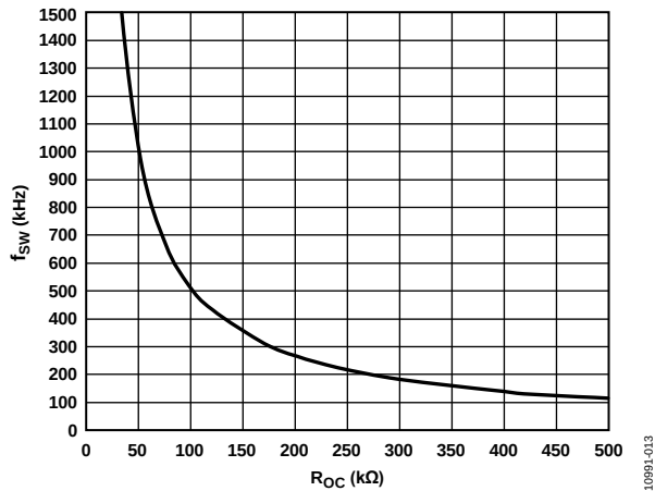
Figure 13. Switching Frequency ( f_{SW} ) vs. R_{OC} Resistance
