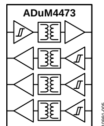
Figure 5. ADuM4473
