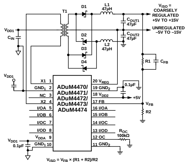
Figure 50. Positive and Unregulated Negative Supply
