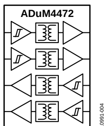
Figure 4. ADuM4472
