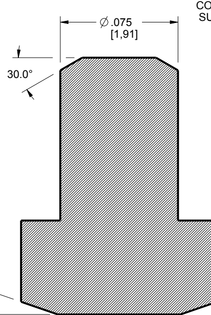
SECTION X-X
