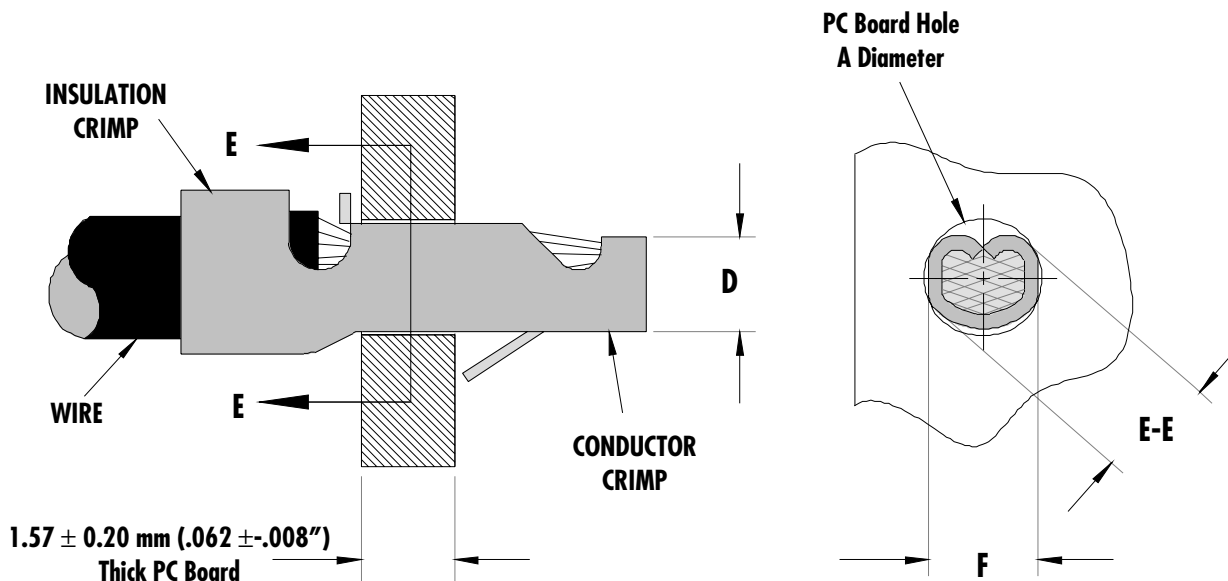
Section E-E
