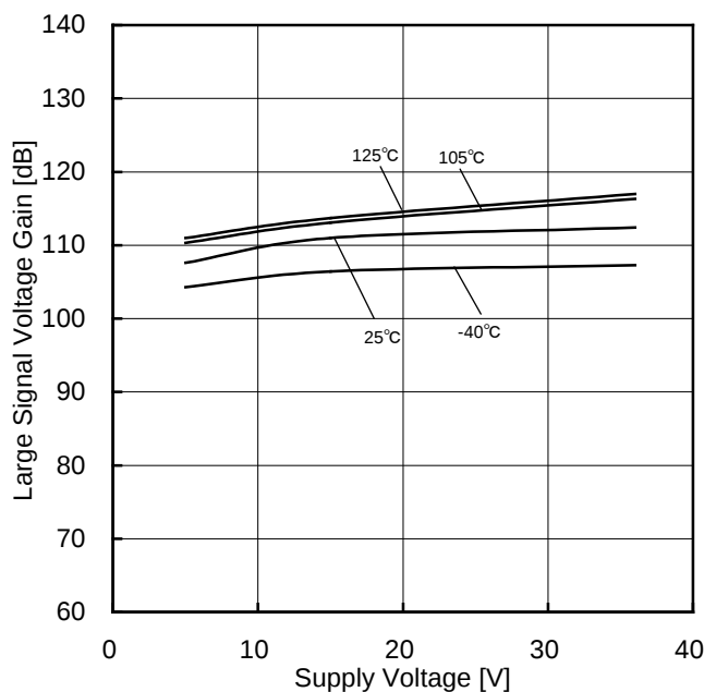
Figure 101. Large Signal Voltage Gain vs Supply Voltage
