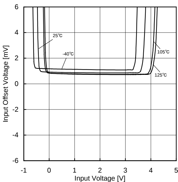
Figure 82. Input Offset Voltage - Input Voltage (VCC=5V)
