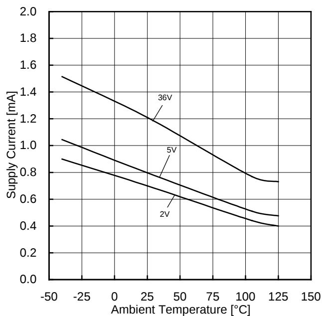
Figure 90. Supply Current vs Ambient Temperature
