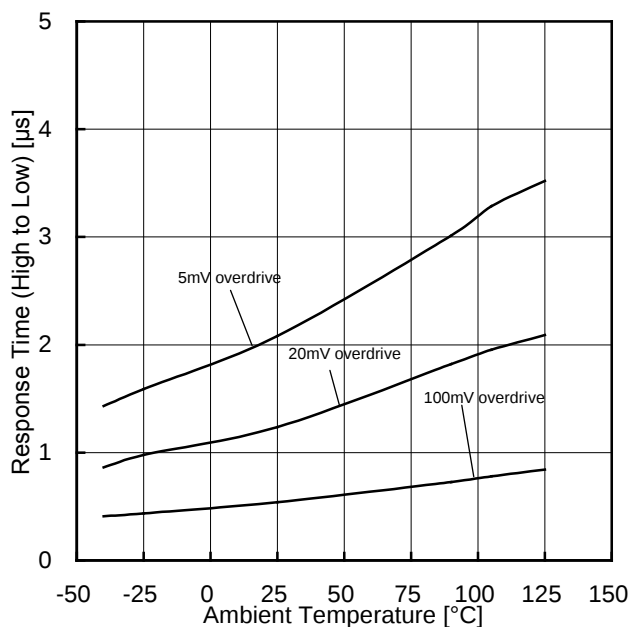
Figure 110. Response Time (High to Low) vs Ambient Temperature ( V_{CC}=5\text{V} , V_{RL}=5\text{V} , R_L=5.1\text{k}\Omega )
