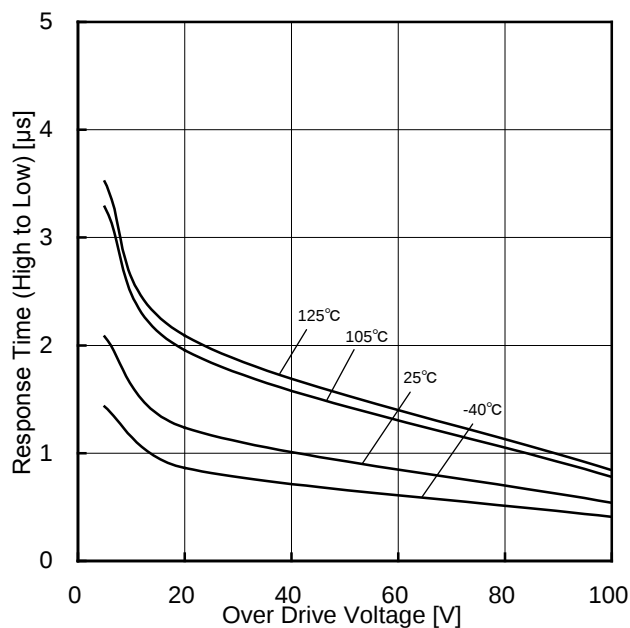
Figure 109. Response Time (High to Low) vs Over Drive Voltage ( V_{CC}=5\text{V} , V_{RL}=5\text{V} , R_L=5.1\text{k}\Omega )
