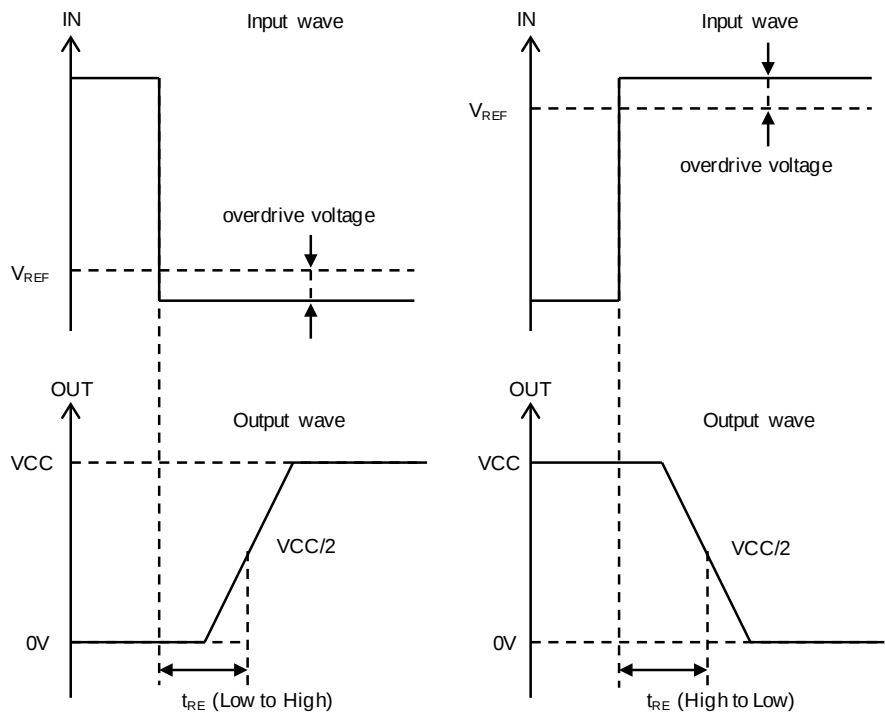
Figure 113. Response Time
