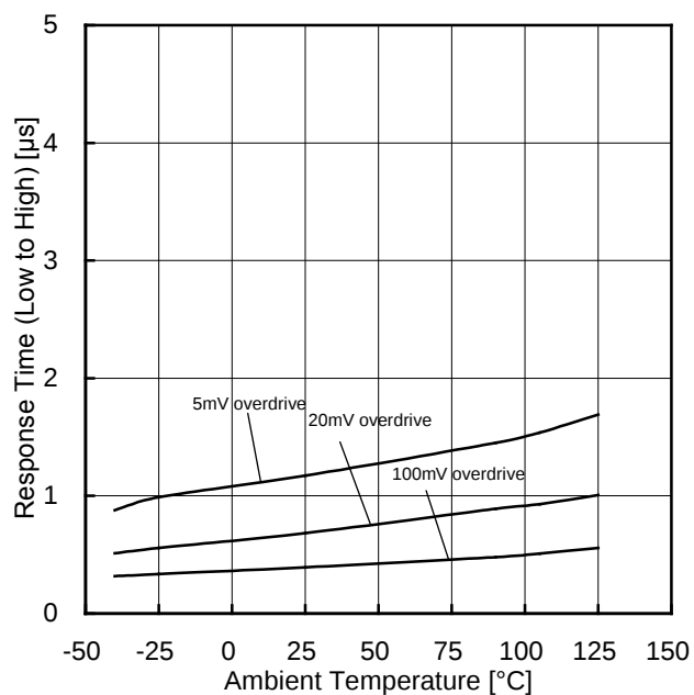
Figure 108. Response Time (Low to High) vs Ambient Temperature ( V_{CC}=5\text{V} , V_{RL}=5\text{V} , R_L=5.1\text{k}\Omega )
